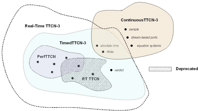
Fig. 2. TTCN-3 overview of proposed extensions
